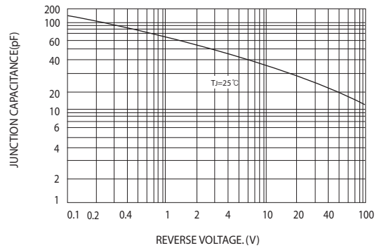
FIG.4-TYPICAL JUNCTION CAPACITANCE
